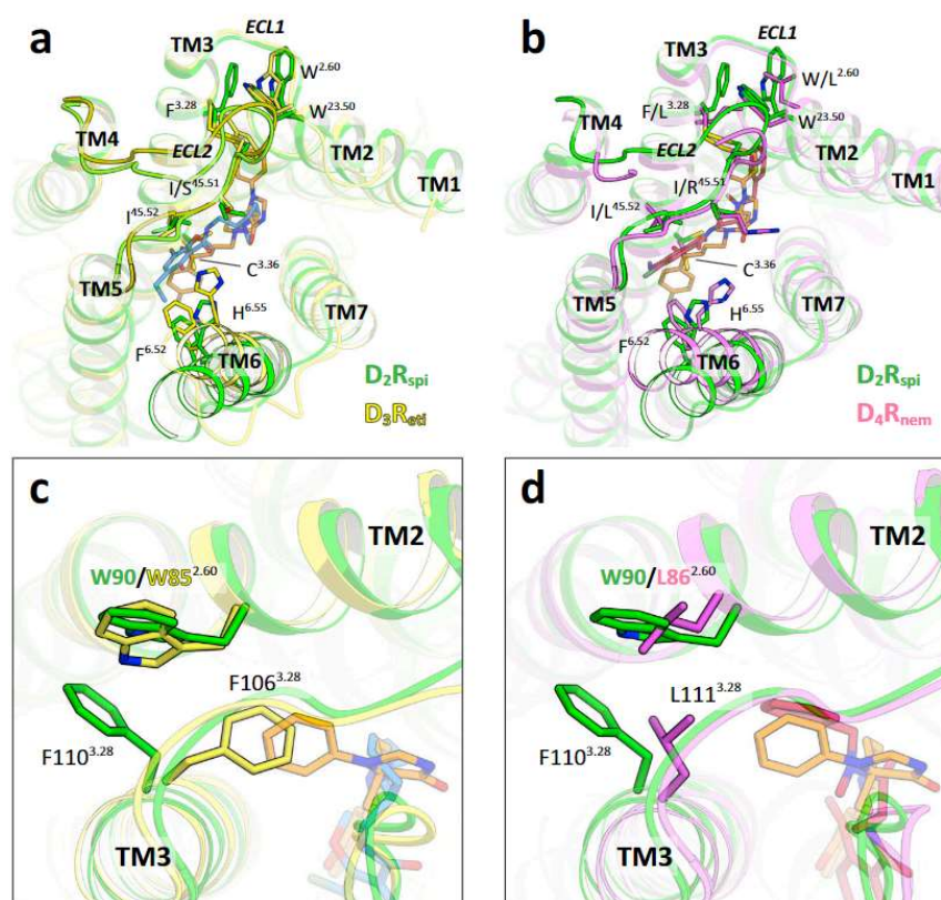
Fig. 5 Comparison of D_2R_{spi} , D_3R_{eti} and D_4R_{nem} . Extracellular view of the superpositions of D_2R_{spi} and either D_3R_{eti} (a) or D_4R_{nem} (b). c The EBP of D_2R_{spi} and the corresponding part of D_3R_{eti} . d Superposition of the EBP of D_2R_{spi} and D_4R_{nem} . In this figure, D_2R_{spi} (green), D_3R_{eti} (yellow), D_4R_{nem} (pink), spiperone (orange), eticlopride (blue), and nemonapride (red) are shown.
