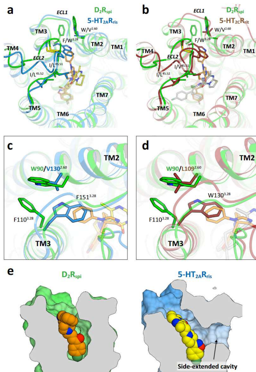
Fig. 4 Comparison of D_2R_{spi} and 5-HT_2 receptors. Extracellular view of the superpositions of D_2R_{spi} and either 5-HT_{2A}R_{ris} ( a ) or 5-HT_{2C}R_{rit} ( b ). c The EBP of D_2R_{spi} and the corresponding part of 5-HT_{2A}R_{ris} . d The EBP of D_2R_{spi} and the corresponding part of 5-HT_{2C}R_{rit} . e Vertical cross sections of D_2R_{spi} and 5-HT_{2A}R_{ris} . In this figure, D_2R_{spi} (green), 5-HT_{2A}R_{ris} (blue), 5-HT_{2C}R_{rit} (brown), spiperone (orange), risperidone (yellow), and ritanserin (gray) are shown.
